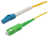
SC/APC to LC/UPC Simplex Singlemode Patch Cord | 123-F1S1-3A356-XX | 123e.com Part Number: 123-F1S1-3A356
